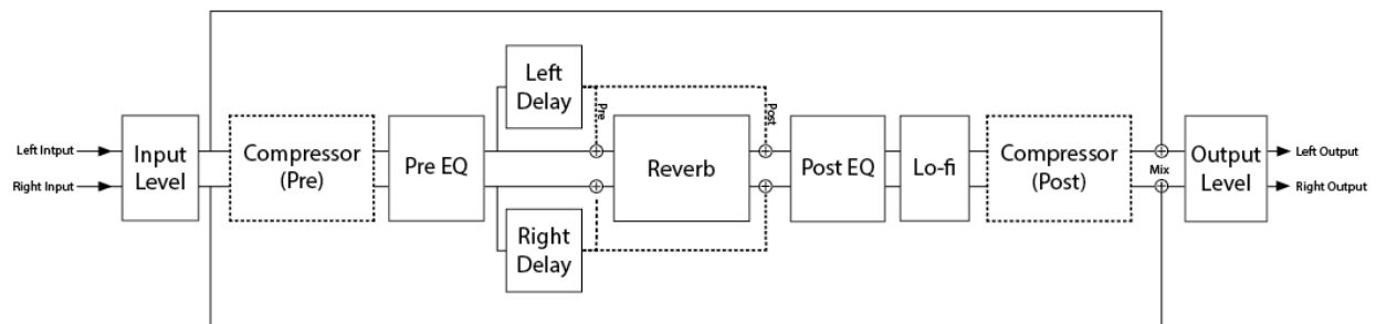
Full Block Diagram
