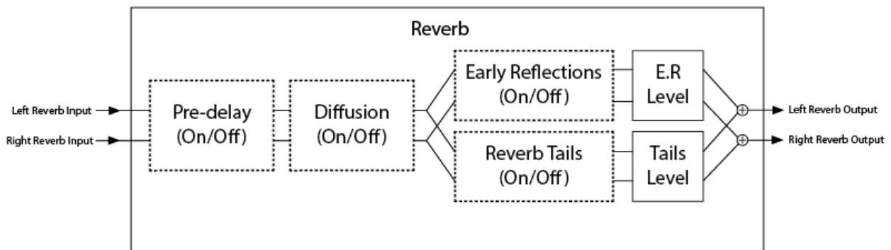
Close-up of the Reverb Block
