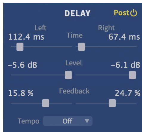
UltraReverb Delay Section
